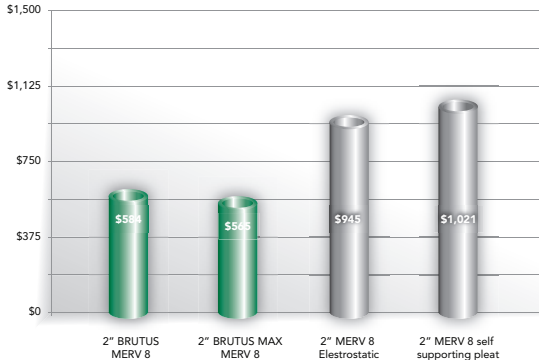
BRUTUS ANNUAL ENERGY COST COMPARISON *
