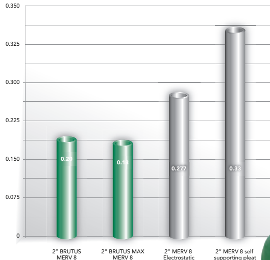
BRUTUS Initial Pressure Drop
